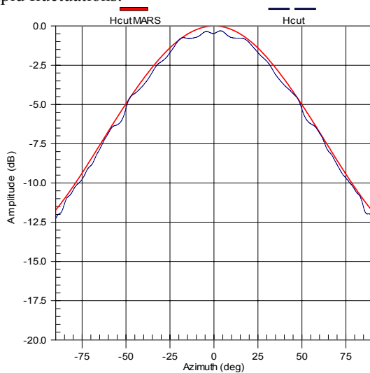
Figure 7. Comparison of azimuth cardinal cuts with and without MARS processing applied
