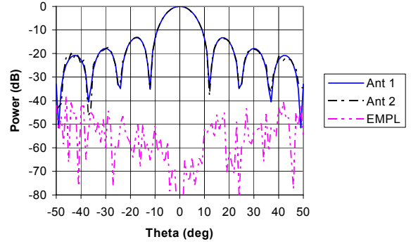
Figure 1. Cuts through Antenna patterns and EMPL.
