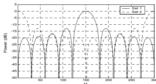
Figure 6. Different patterns with identical histograms
