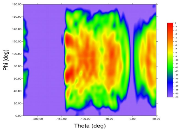
Fig. 9. Far-field transformation from Near-Field measurement with radial correction
