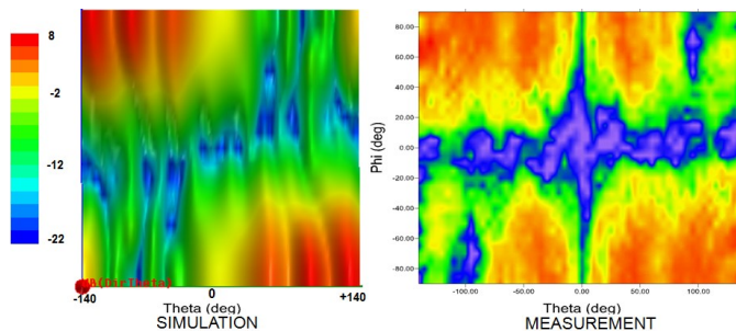
Fig. 5. Comparison between simulated and measured theta gain (dBi) 3D radiation pattern
