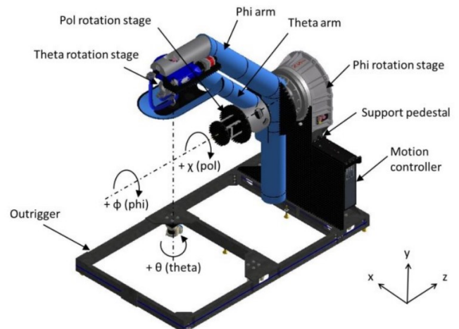
Fig. 1. NSI-700S-360 Articulating 3-axis spherical near-field scanner
