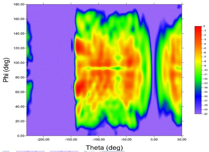
Fig. 8. Far-field transformation from Near-Field measurement without radial correction
