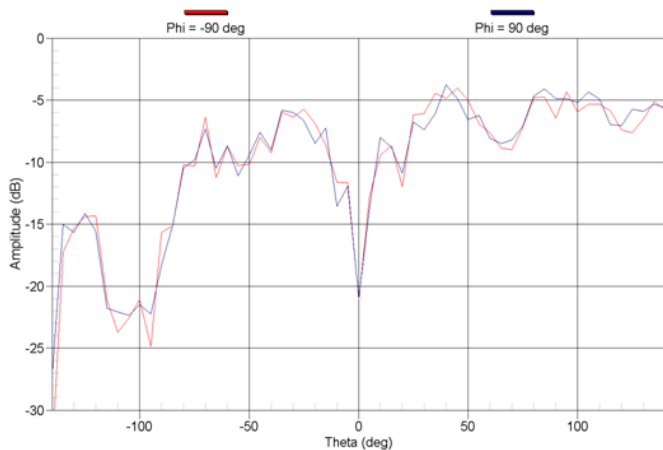
Fig. 6. Near field amplitude on yOz plane for \phi=-90^\circ (red) and \phi=90^\circ (blue) without correction for Copol
