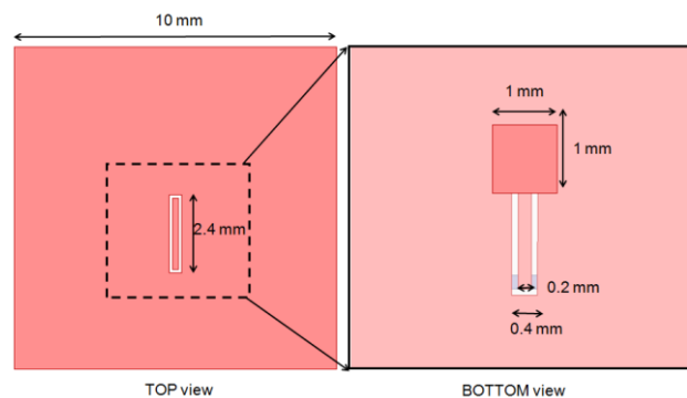
Fig. 4. Antenna dimensions
