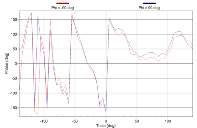
Near field phase on yOz plane for \phi=-90^\circ (red) and \phi=90^\circ (blue) with correction for Copol
