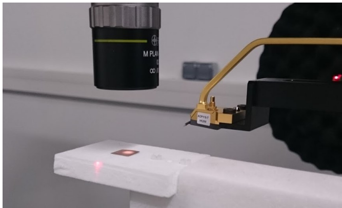
Fig. 2. Waveguide GSG probe and laser alignment of the AUT
