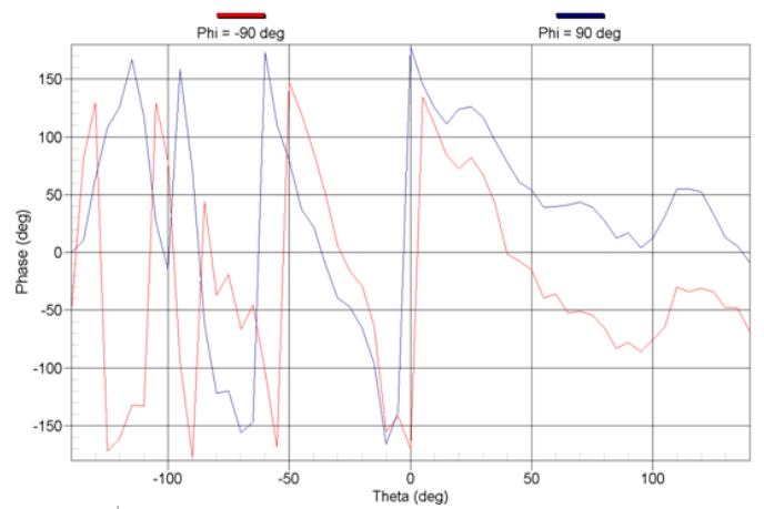
Fig. 7. Near field phase on yOz plane for \phi=-90^\circ (red) and \phi=90^\circ (blue) without correction for Copol
